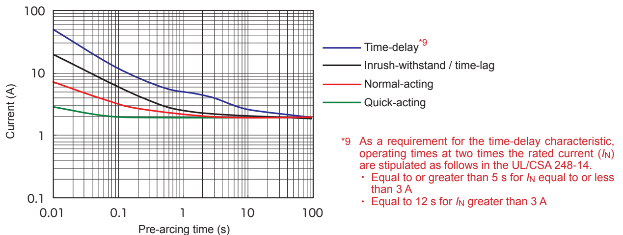
Figure 7 - Imaginal figure to explain differences in pre-arcing-time current characteristics for the same rated current
